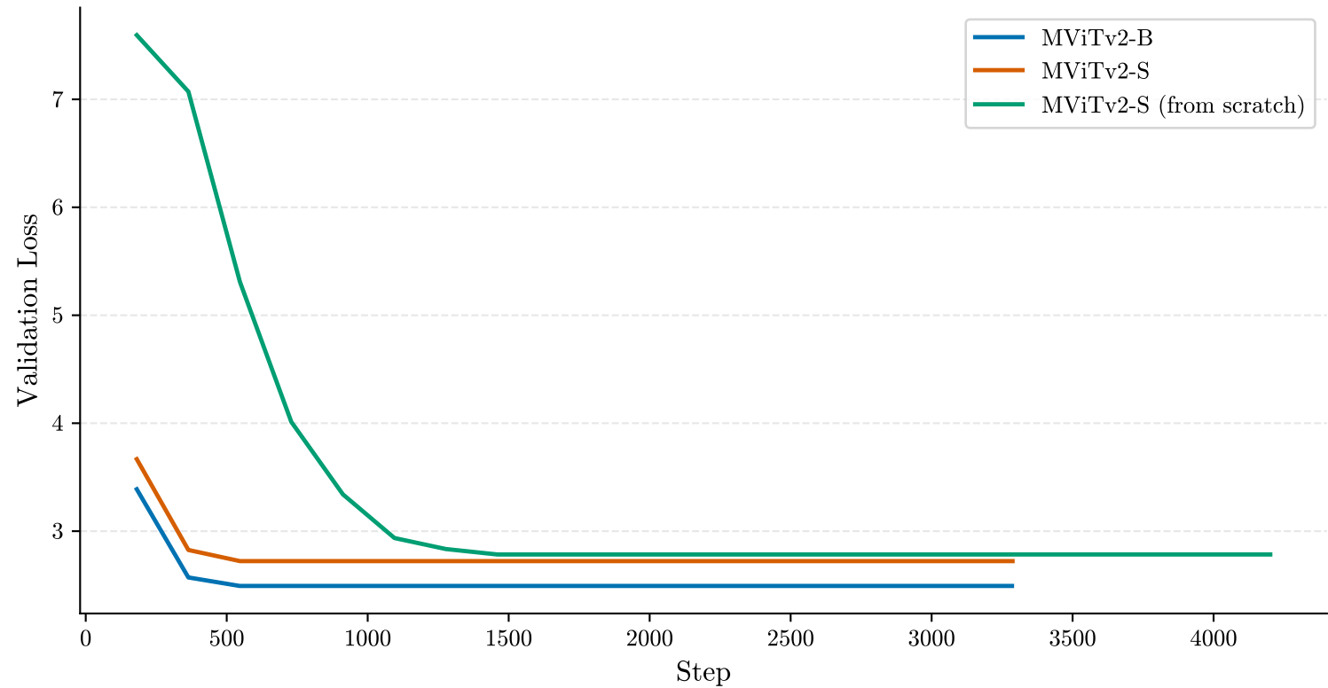
Best Validation Loss vs Step
